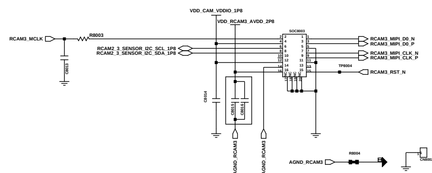
RCAM3_2M MACRO CAMERA(16PIN)
