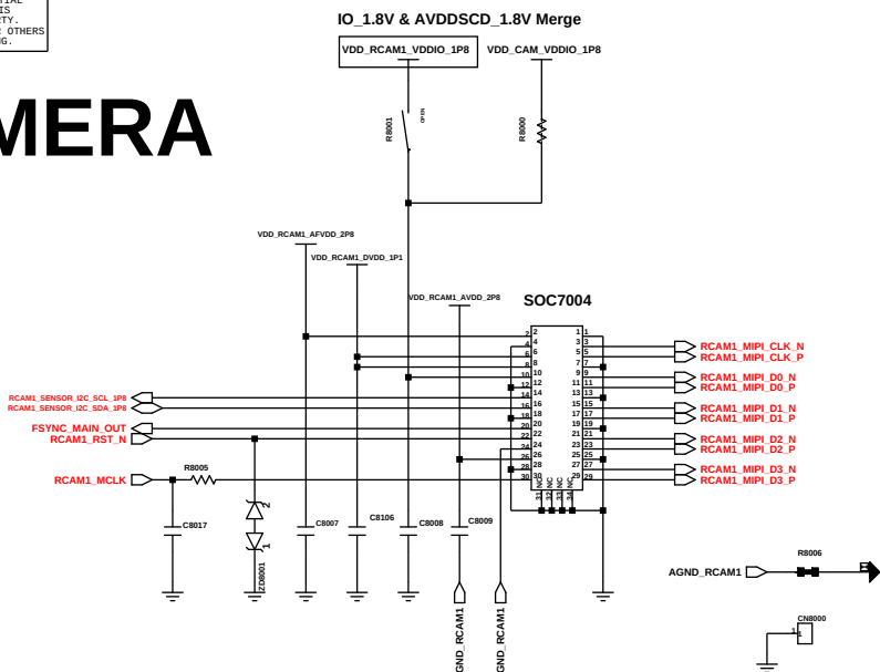
RCAM1_50M(30PIN) (A04S CAM pin map)
